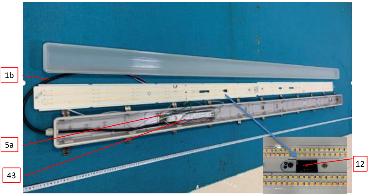
Photo 40 - LED PCB view of model TS-TPL3-8FT70W-X-TCP(XX).
