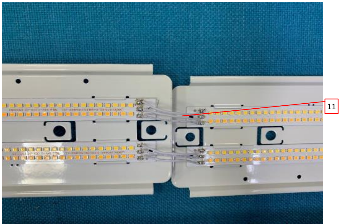
Photo 40 - LED PCB view of model TS-TPL3-8FT70W-X-TCP(XX).
