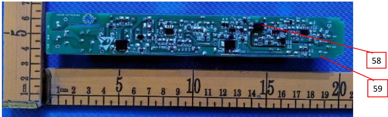
Photo 47 - Trace side view of LED driver 9.
