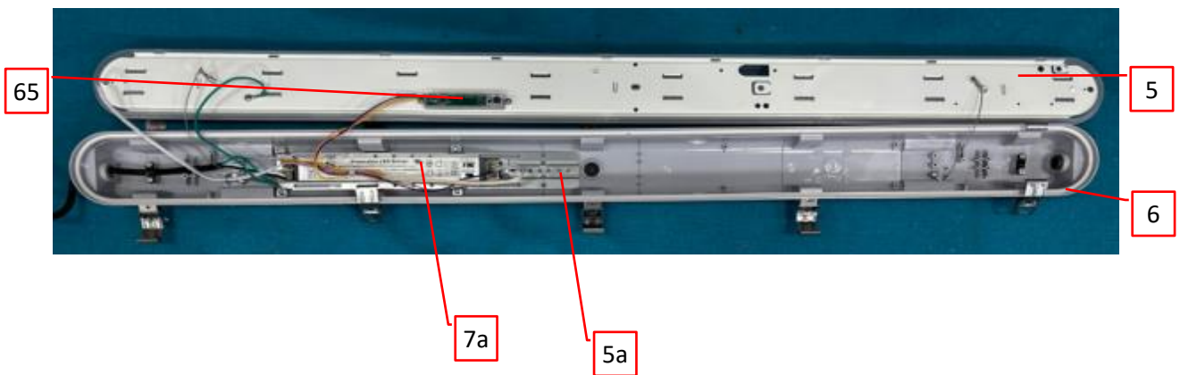
Photo 4a - Internal view of model TS-TPL1-4FT30W/40W/50W-X-TCP(MS)
