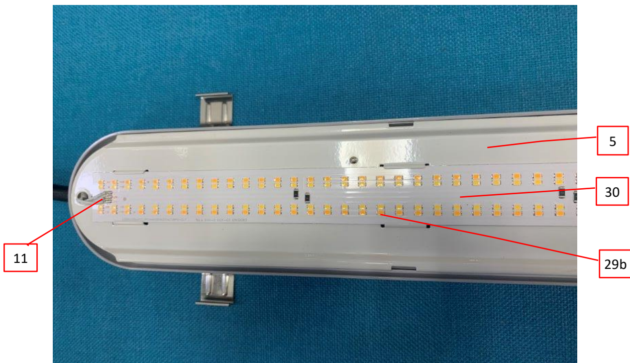
Photo 55 - LED PCB view of model TS-TPL1-4FT30W/40W/50W-X-347-TCP(XX).
