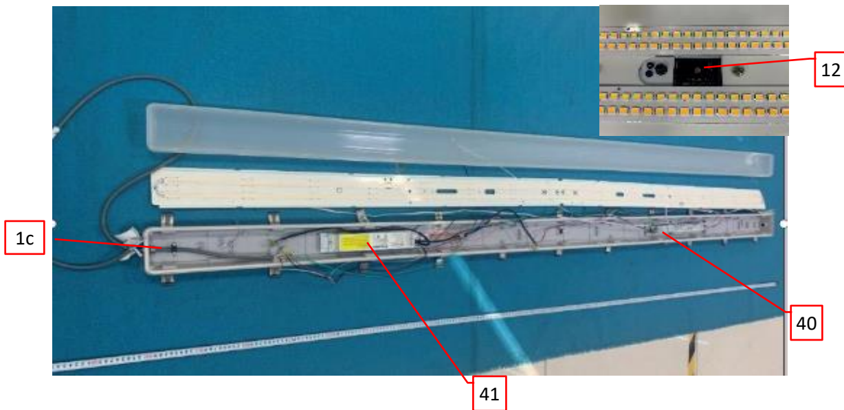
Photo 38 - Closed-up view of model TS-TPL3-8FT70W-X-TCP(EM) and TS-TPL3-8FT70W-X-TCP(EMS), also represent for models TS-TPL3-4FT50W-X-TCP(EM) and TS-TPL3-4FT50W-X-TCP(EMS)
