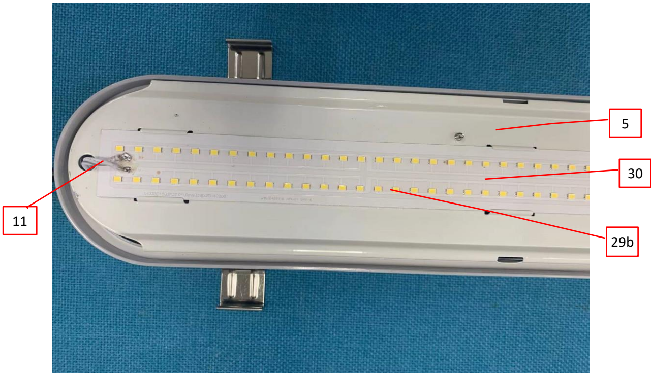
Photo 56 - LED PCB view of model TS-TPL1-4FT32W-X-XXK(XX).
