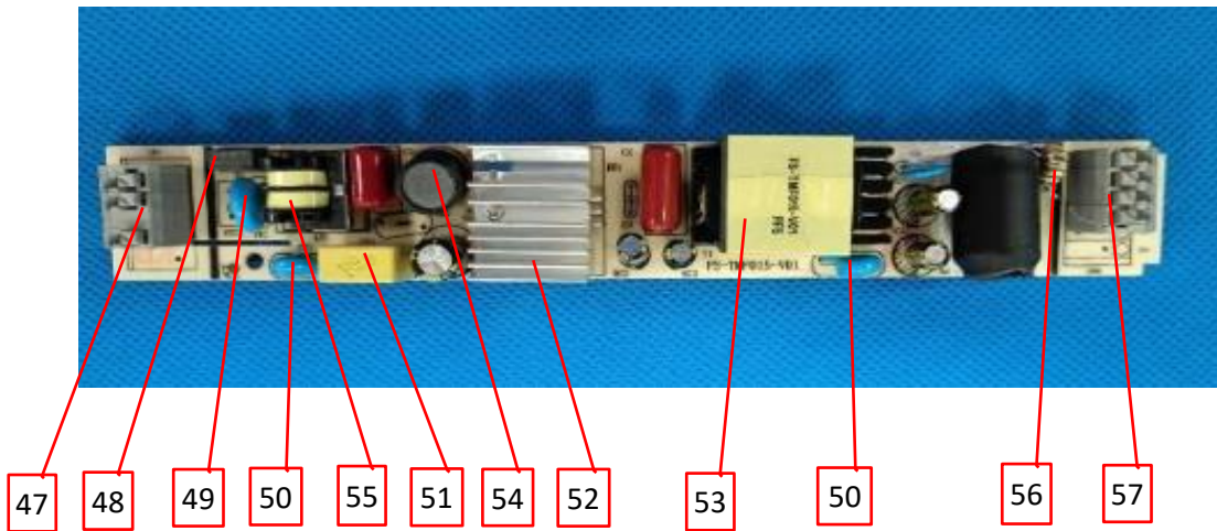
Photo 46a - Component side view of LED driver 9.
