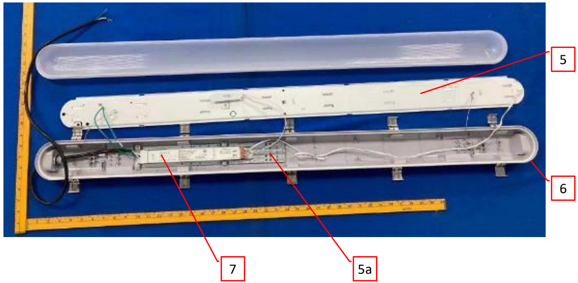
Photo 4a - Internal view of model TS-TPL1-4FT30W/40W/50W-X-TCP(MS)
