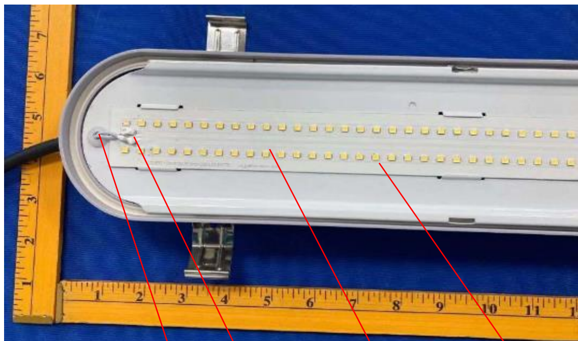
Photo 18 - LED PCB view of model TS-TPL1-4FT40W-X-347-XXK(XX)
