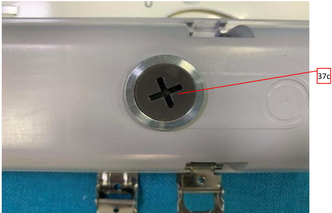
Photo 35 - Closed-up view of model TS-TPL1-4FT40W-X-XXK, also represent of models TS-TPL3-4FT50W-X-TCP(XX), TS-TPL3-8FT70W-X-TCP(XX).
