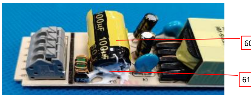
Photo 46b - Alternative component side view of LED driver 9.
