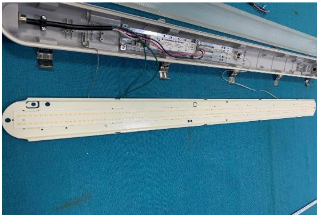
Photo 32 - Internal view of model TS-TPL1-4FT40W-X-XXK.
