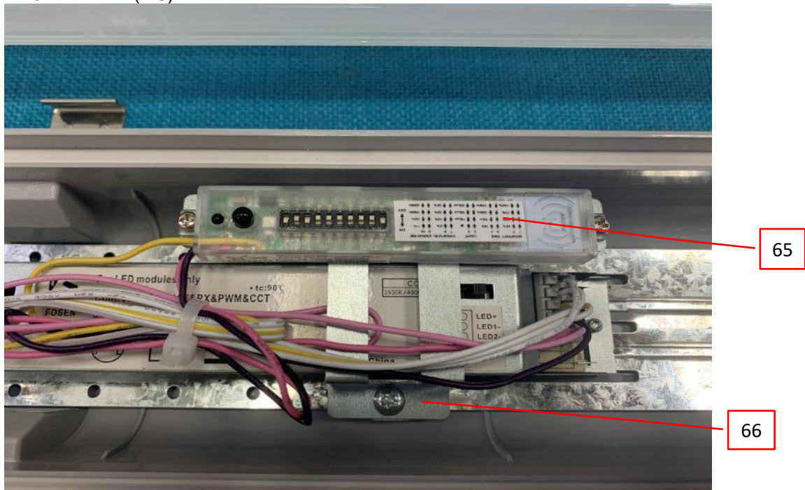
Photo 59 - Internal view of sensor-3.
