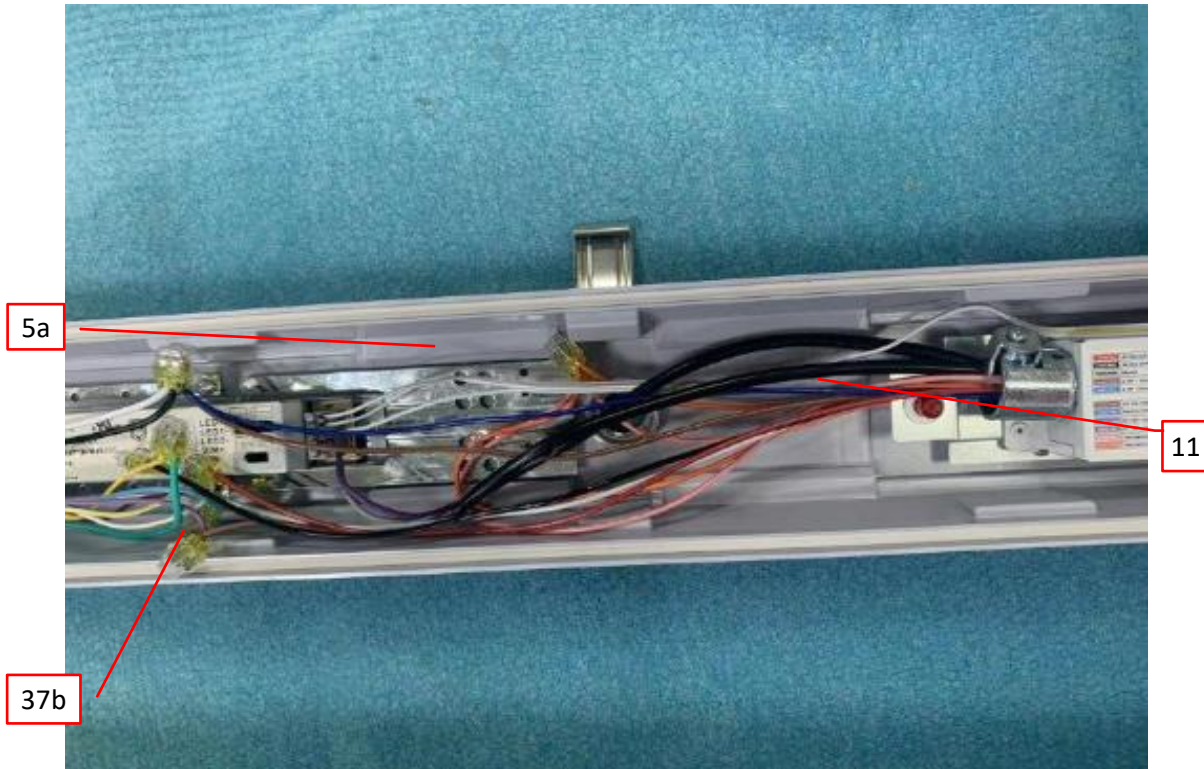
Photo 38 - Closed-up view of model TS-TPL3-8FT70W-X-TCP(EM) and TS-TPL3-8FT70W-X-TCP(EMS), also represent for models TS-TPL3-4FT50W-X-TCP(EM) and TS-TPL3-4FT50W-X-TCP(EMS)
