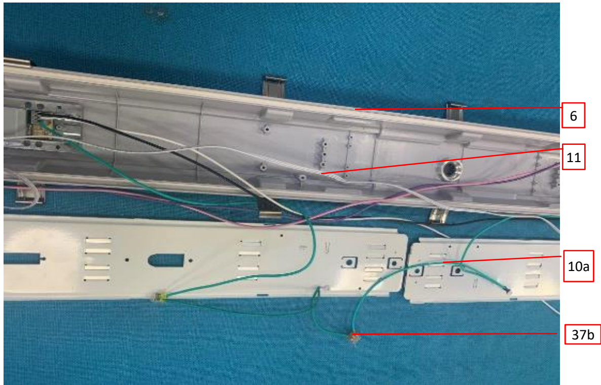
Photo 41 - Bonding and internal view of model TS-TPL3-8FT70W-X-TCP(XX).
