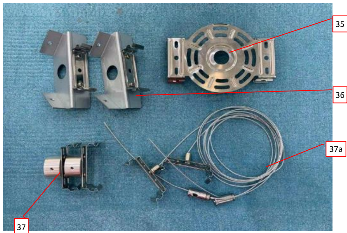
Photo 43 - Mounting accessories view of models TS-TPL1-4FT40W-X-XXK, TS-TPL3-2FT20W-X-TC(XX), TS-TPL3-4FT50W-X-TCP(XX), TS-TPL3-8FT70W-X-TCP(XX), TS-TPL3-4FT40W-X-XXK, TS-TPL3-8FT70W-X-XXK, TS-TPL1-4FT30W/40W/50W-X-347-TCP(XX), TS-TPL1-4FT32W-X-XXK(XX), TS-TPL3-2FT25W-X-TCP(XX), TS-TPL3-4FT80W-X-TCP(XX), TS-TPL3-8FT100W-X-TCP(XX), TS-TPL3-2FT20W-X-347-TC(XX), TS-TPL3-4FT50W-X-347-TCP(XX), TS-TPL3-8FT70W-X-347-TCP(XX)
