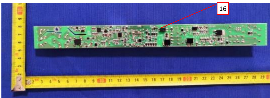
Photo 24 - Trace side view of LED driver 3.
