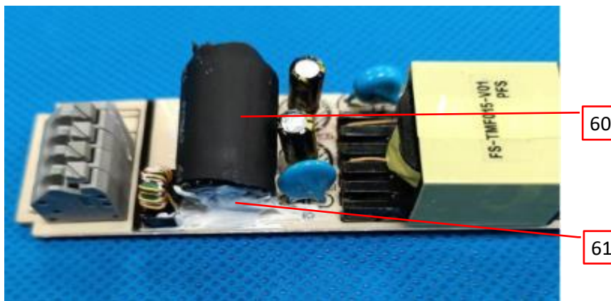
Photo 46b - Alternative component side view of LED driver 9.
