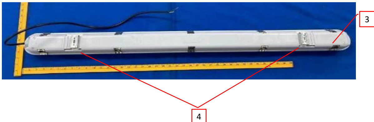
Photo 2 - Rear view of models TS-TPL1-4FT40W-X-347-XXK(XX), TS-TPL1-4FT30W/40W/50W-X-TCP(XX) and TS-TPL1-4FT25W/30W/40W-X-TCP.
