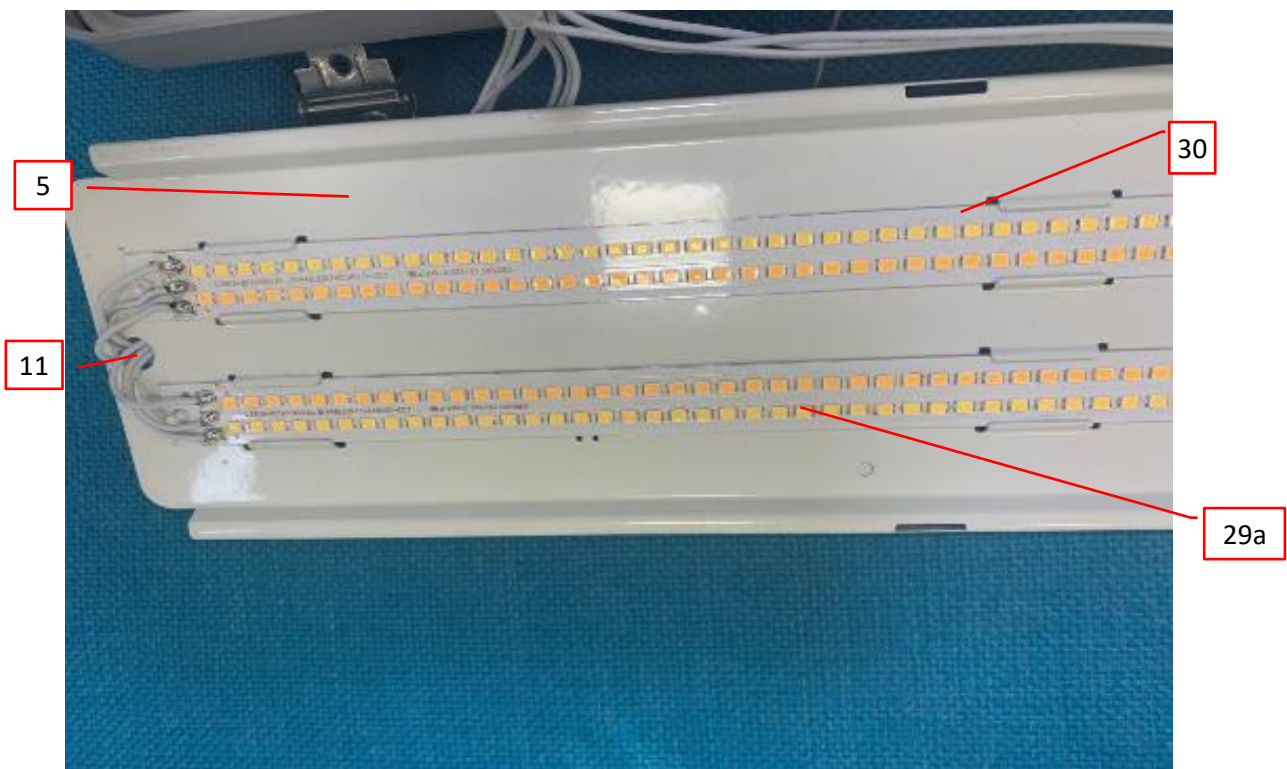
Photo 42 - LED PCB view of model TS-TPL3-8FT70W-X-TCP(XX), also represent of models TS-TPL3-2FT20W-X-TC(XX) and TS-TPL3-4FT50W-X-TCP(XX), TS-TPL3-4FT40W-X-XXK, TS-TPL3-8FT70W-X-XXK
