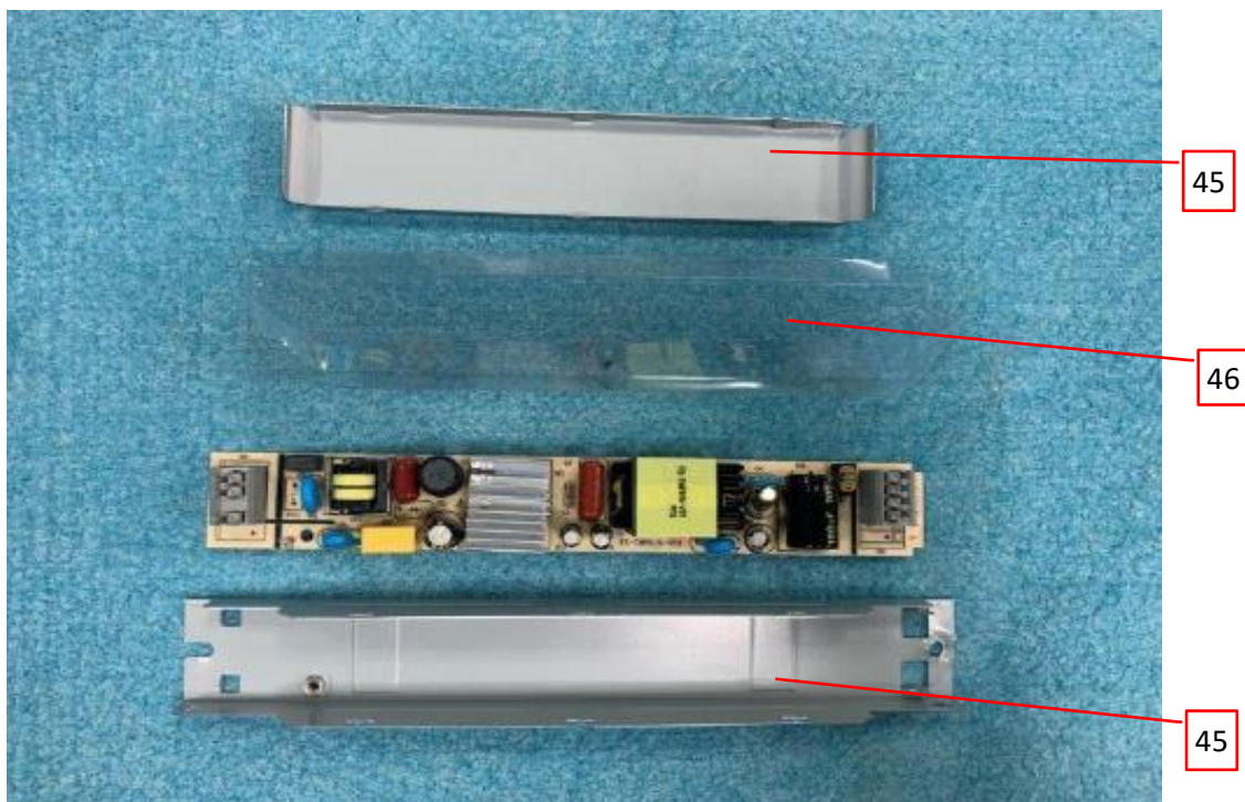
Photo 45 - Internal view of LED driver 9.
