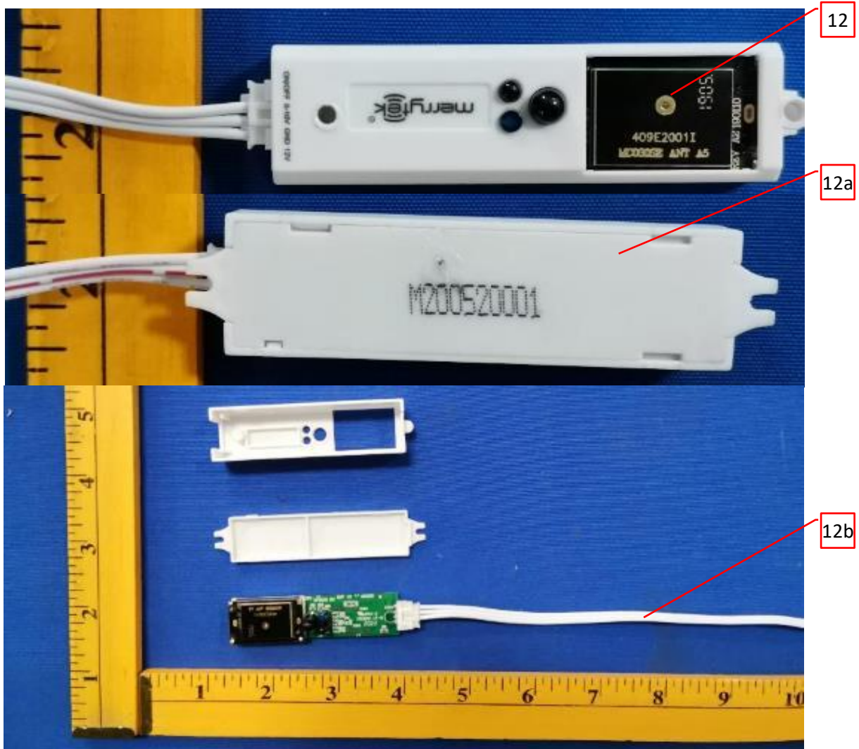
Photo 12 - Sensor PCB view of sensor model MC090D RC
