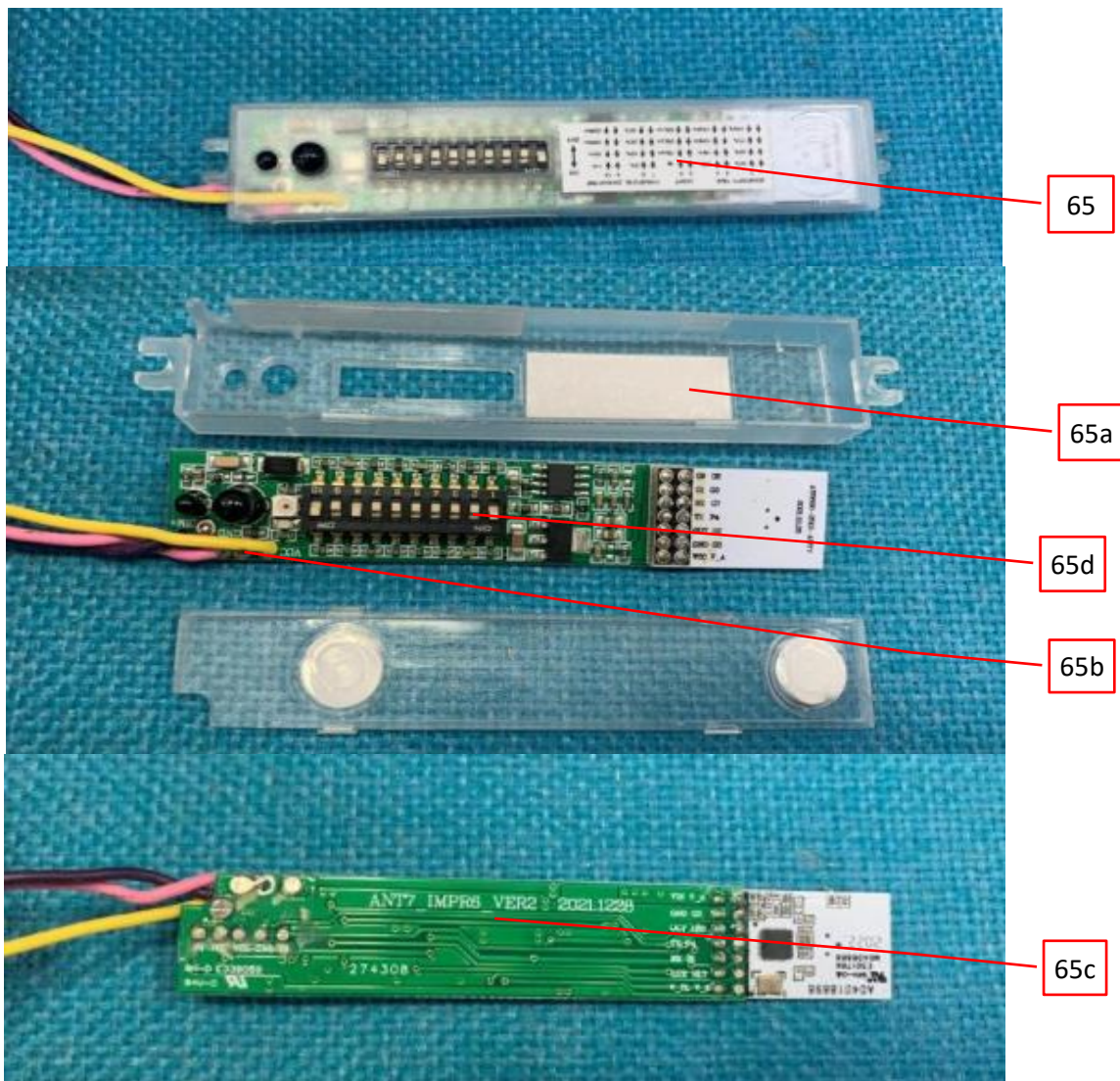
Photo 59 - Internal view of sensor-3.
