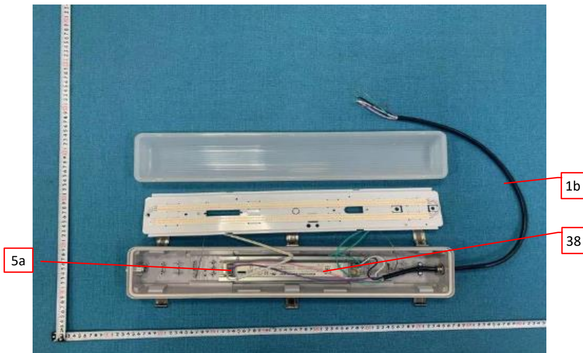
Photo 36 - Internal view of model TS-TPL3-2FT20W-X-TC.
